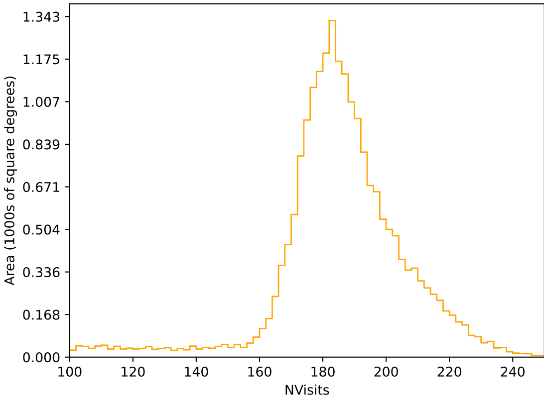
too_elab_r64_d3_giz_v3.4_10yrs All sky r band: NVisits
