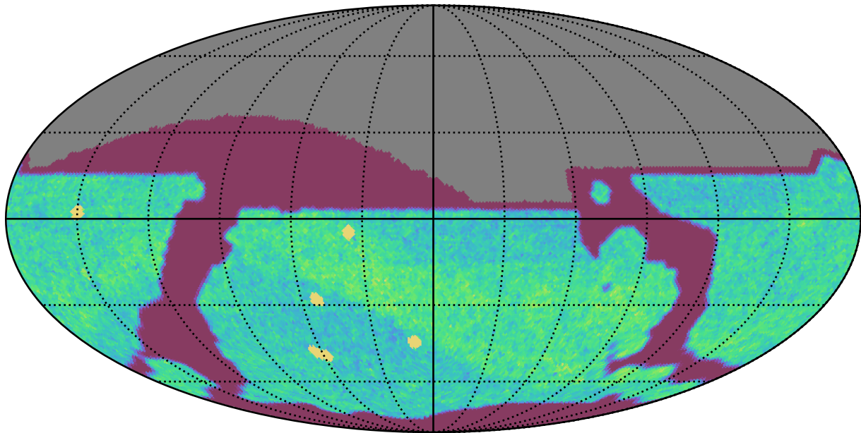
too_elab_r64_d3_giz_v3.4_10yrs All sky i band: NVisits
