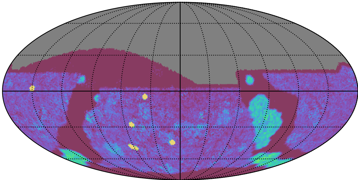
too_elab_r64_d3_giz_v3.4_10yrs All sky g band: NVisits
