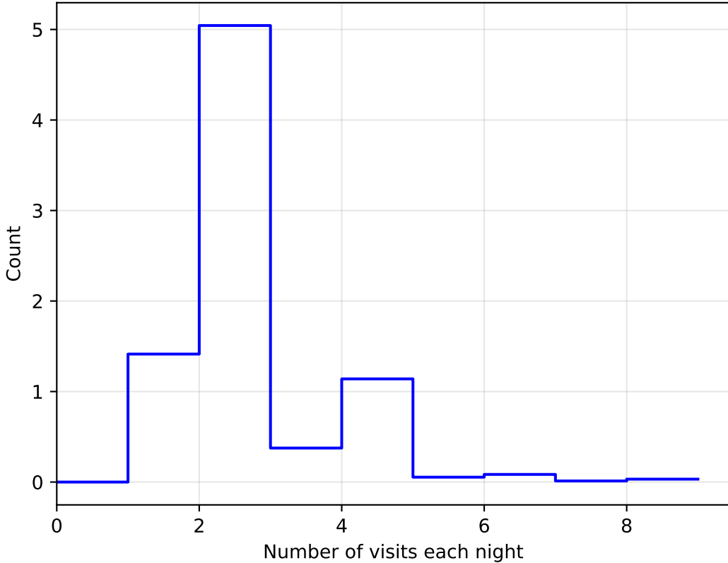
too_elab_r64_d3_giz_v3.4_10yrs WFD: NVisitsPerNight
