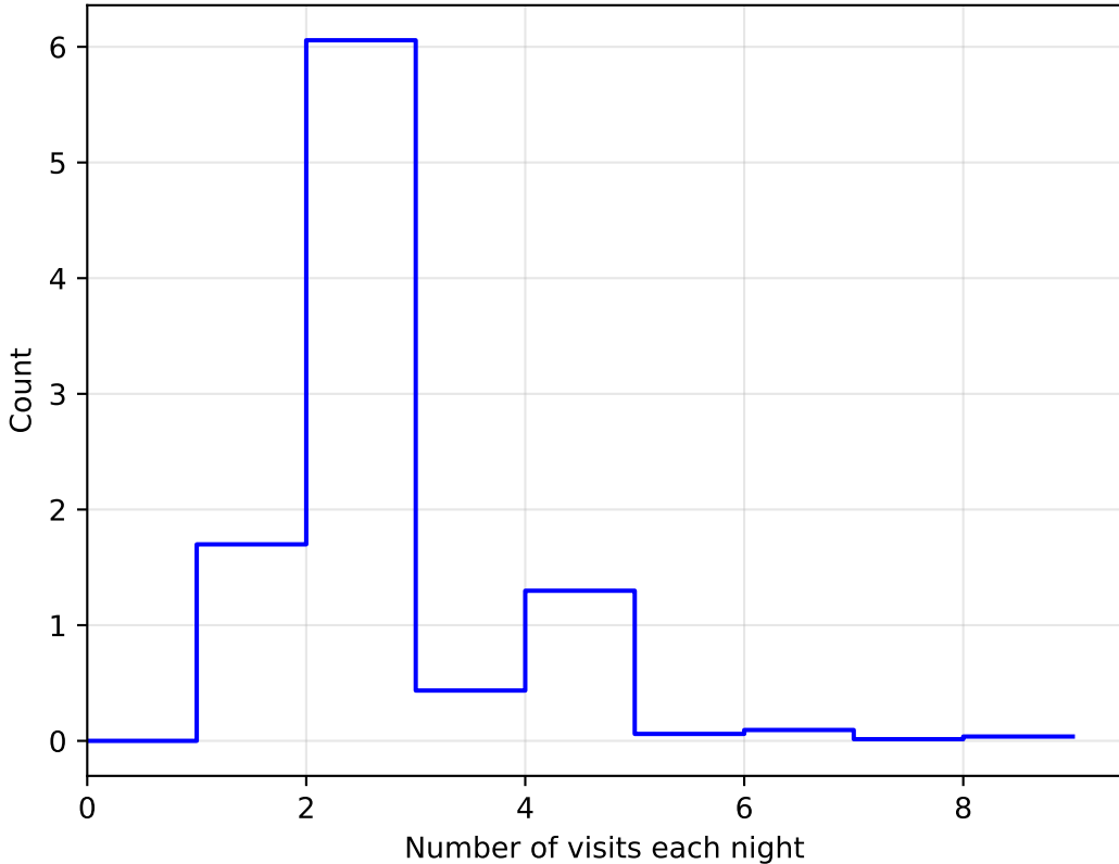
too_elab_r64_d3_giz_v3.4_10yrs All sky: NVisitsPerNight
