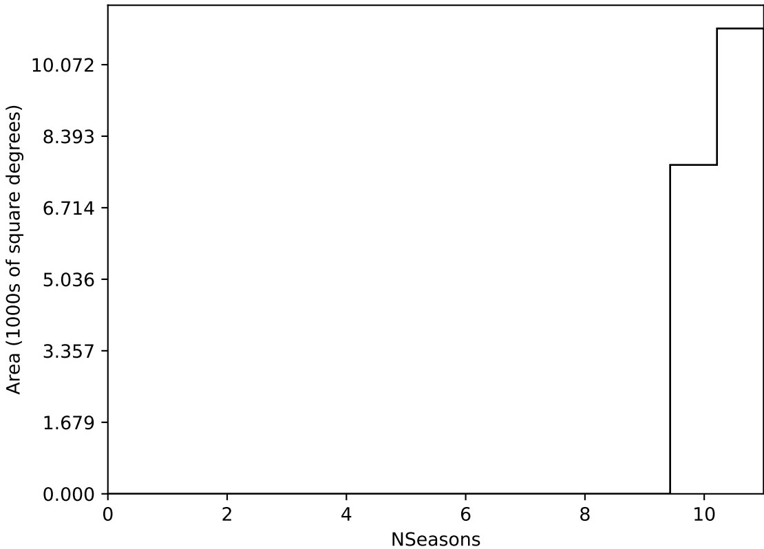
too_elab_r64_d3_giz_v3.4_10yrs WFD all bands: NSeasons
