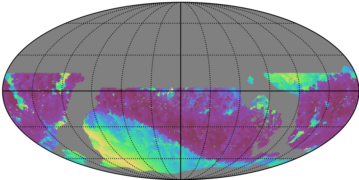
too_elab_r64_d3_giz_v3.4_10yrs WFD z band: Min solarElong
