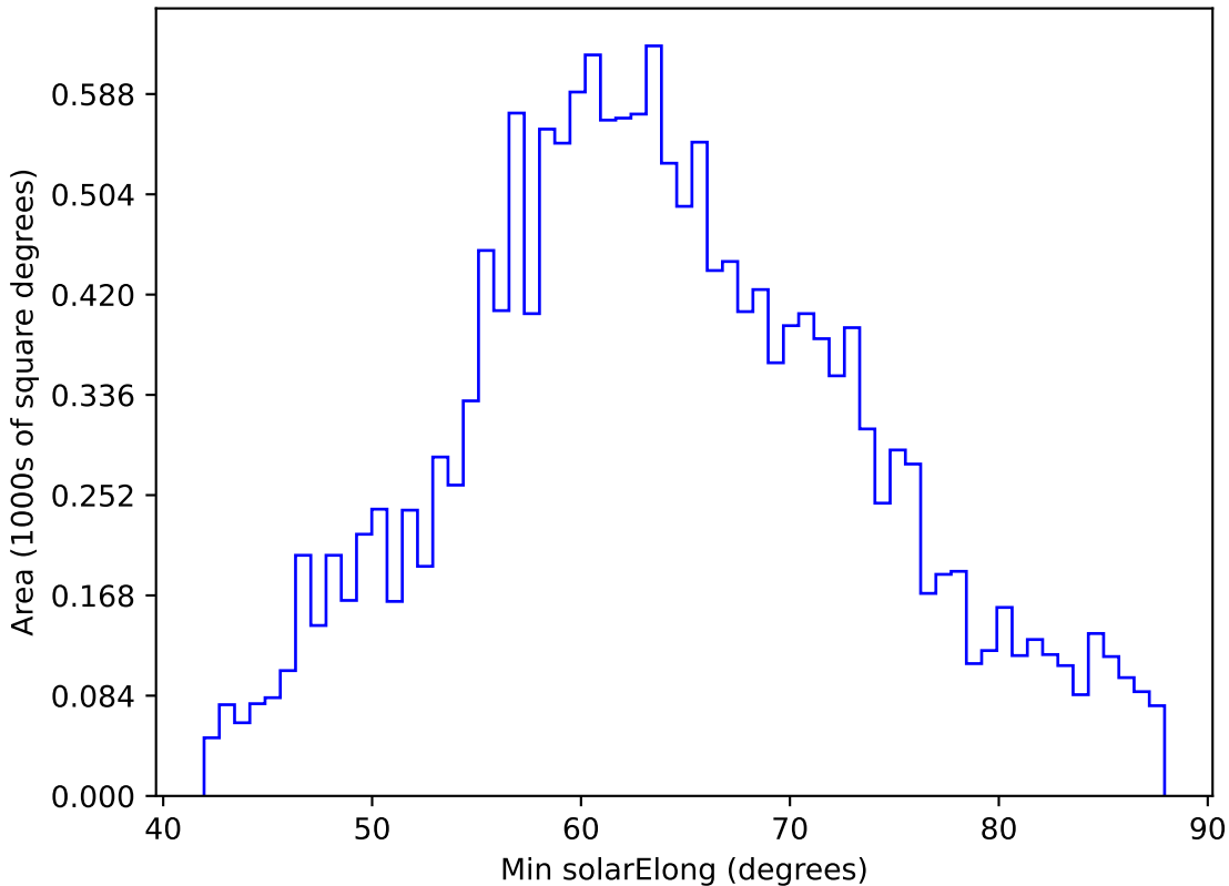
too_elab_r64_d3_giz_v3.4_10yrs WFD y band: Min solarElong
