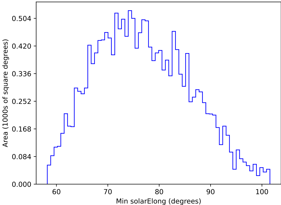
too_elab_r64_d3_giz_v3.4_10yrs WFD u band: Min solarElong
