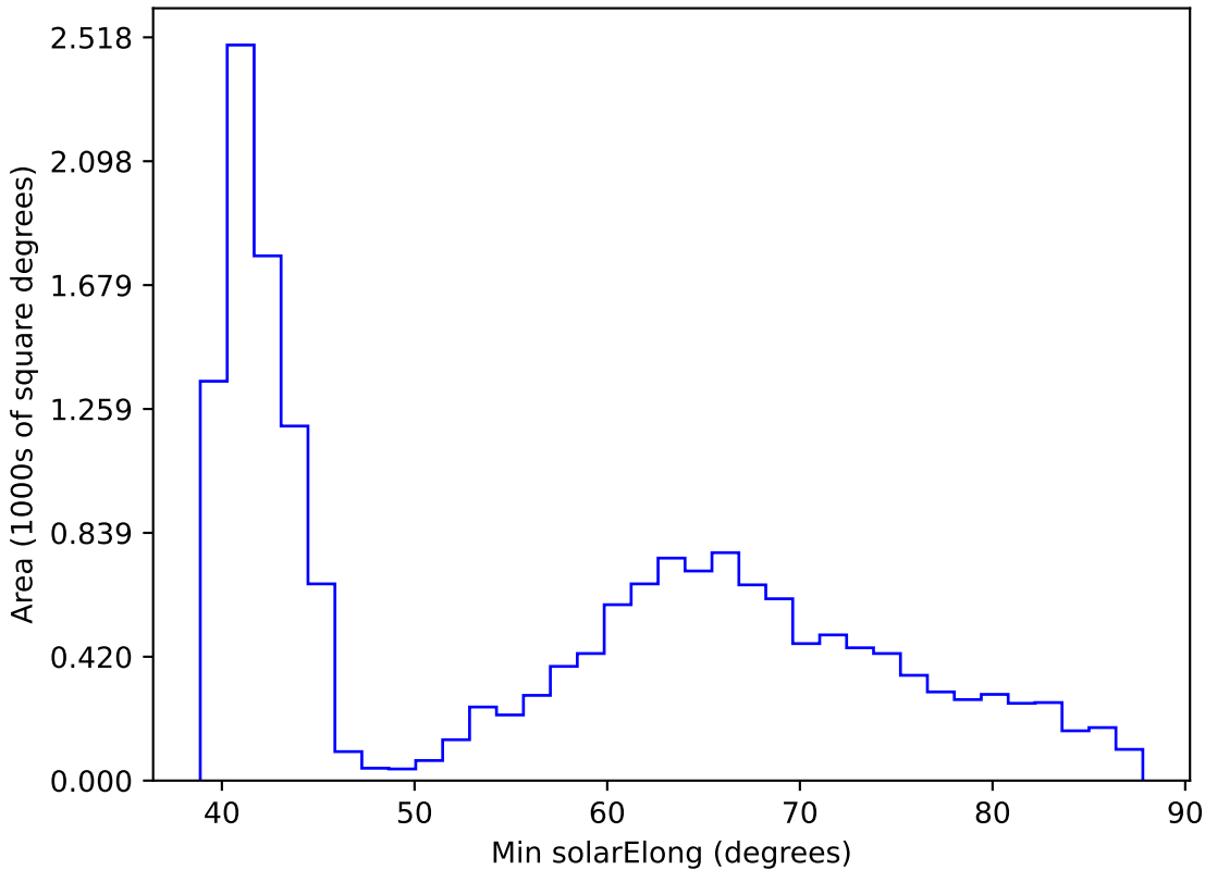
too_elab_r64_d3_giz_v3.4_10yrs WFD r band: Min solarElong
