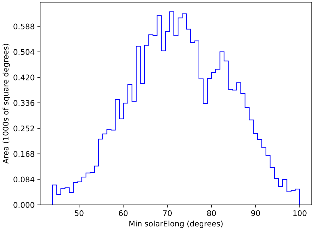
too_elab_r64_d3_giz_v3.4_10yrs WFD g band: Min solarElong
