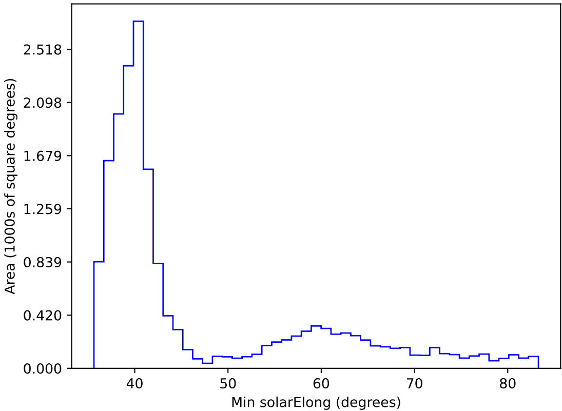
too_elab_r64_d3_giz_v3.4_10yrs WFD all bands: Min solarElong
