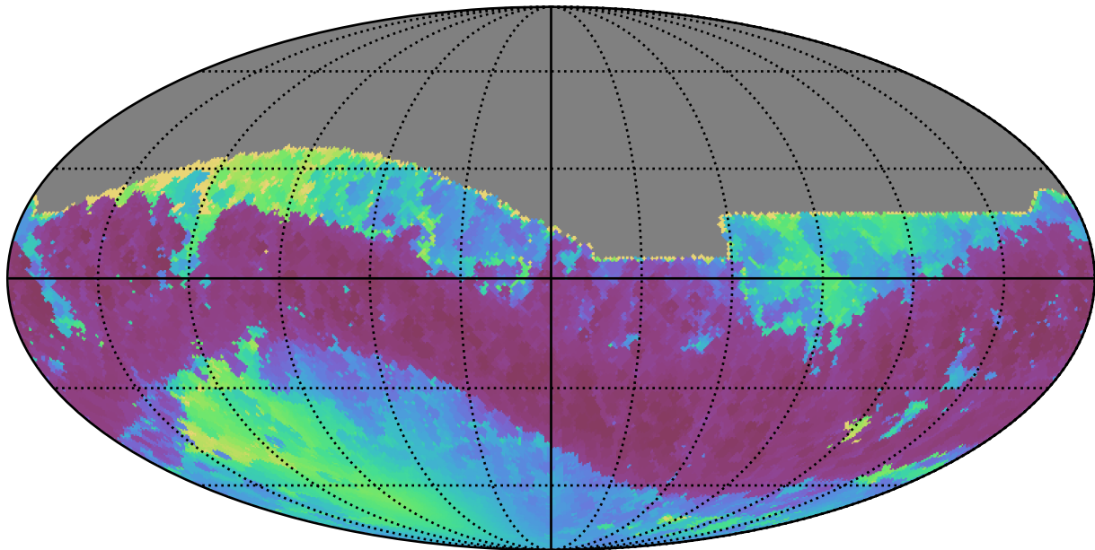
too_elab_r64_d3_giz_v3.4_10yrs All sky z band: Min solarElong
