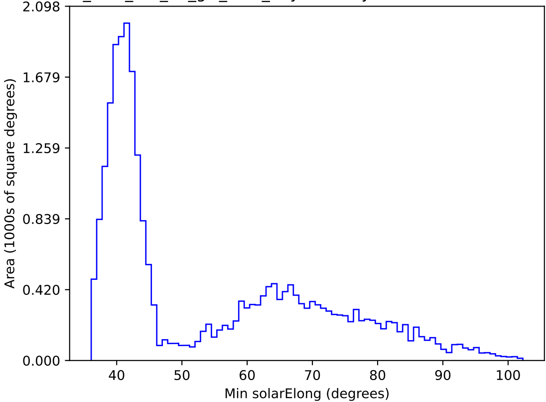
too_elab_r64_d3_giz_v3.4_10yrs All sky z band: Min solarElong
