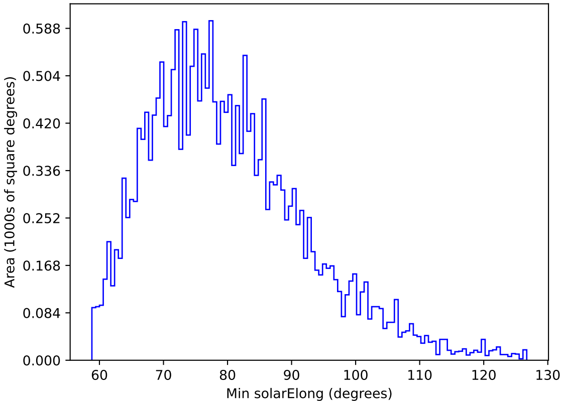
too_elab_r64_d3_giz_v3.4_10yrs All sky u band: Min solarElong
