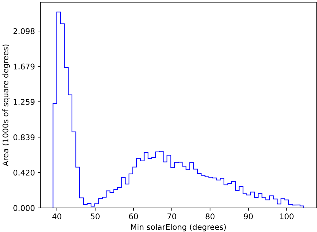
too_elab_r64_d3_giz_v3.4_10yrs All sky r band: Min solarElong
