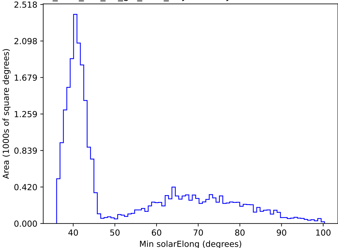
too_elab_r64_d3_giz_v3.4_10yrs All sky i band: Min solarElong
