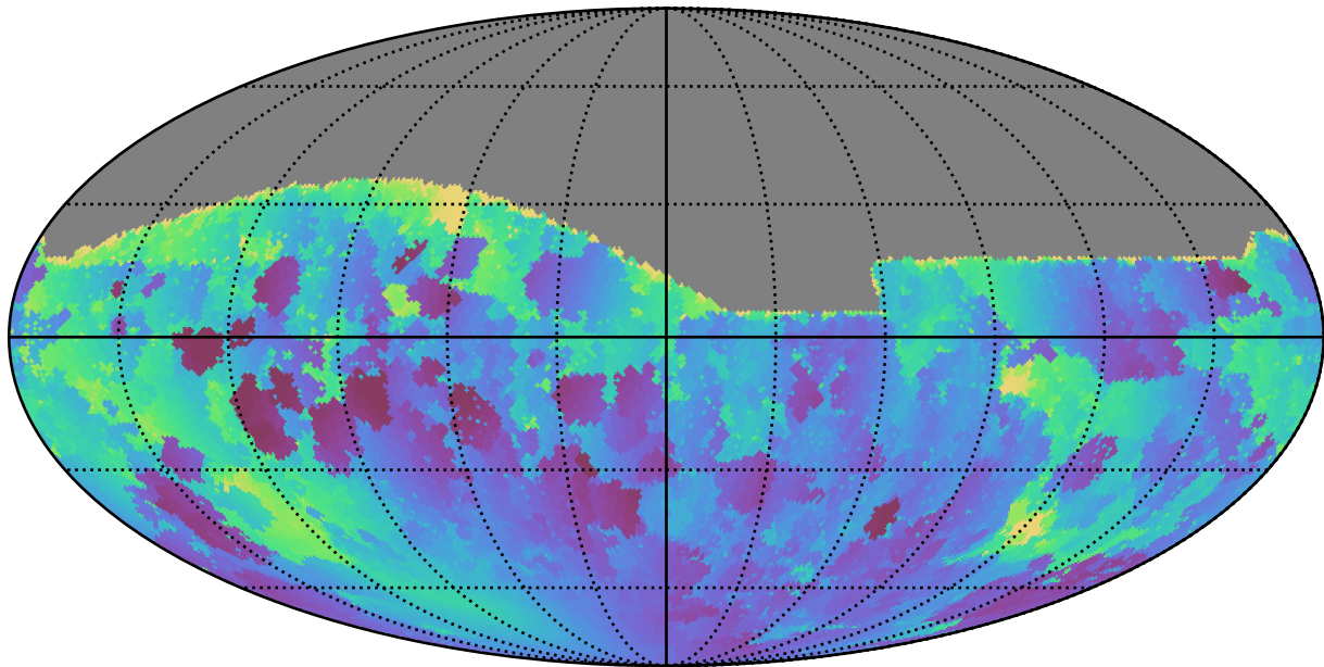
too_elab_r64_d3_giz_v3.4_10yrs All sky g band: Min solarElong
