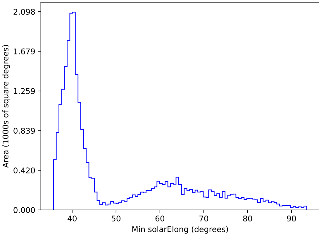
too_elab_r64_d3_giz_v3.4_10yrs All sky all bands: Min solarElong
