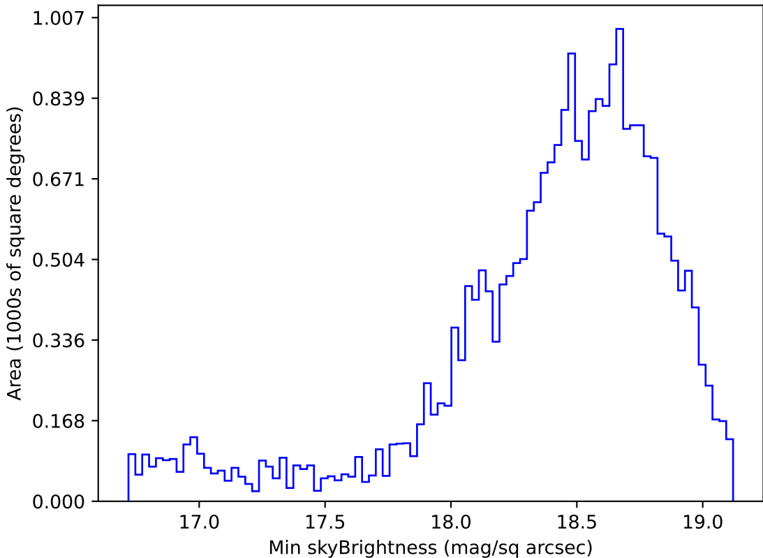
too_elab_r64_d3_giz_v3.4_10yrs Yr 1 z band: Min skyBrightness
