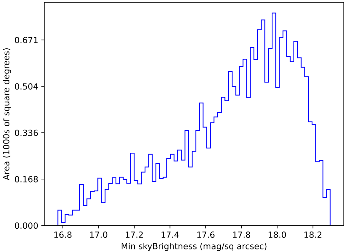
too_elab_r64_d3_giz_v3.4_10yrs Yr 1 y band: Min skyBrightness
