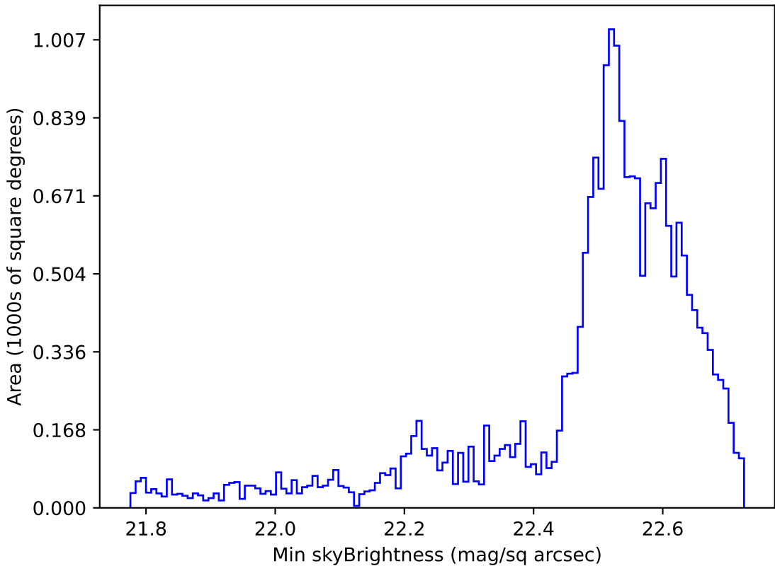
too_elab_r64_d3_giz_v3.4_10yrs Yr 1 u band: Min skyBrightness
