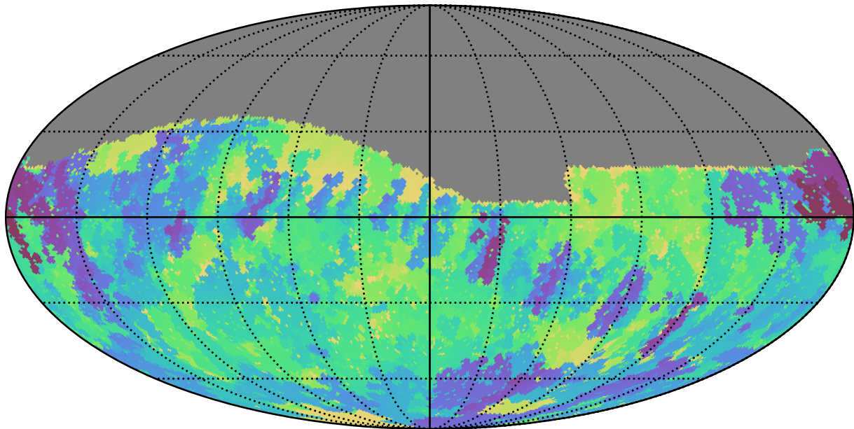
too_elab_r64_d3_giz_v3.4_10yrs Yr 1 r band: Min skyBrightness
