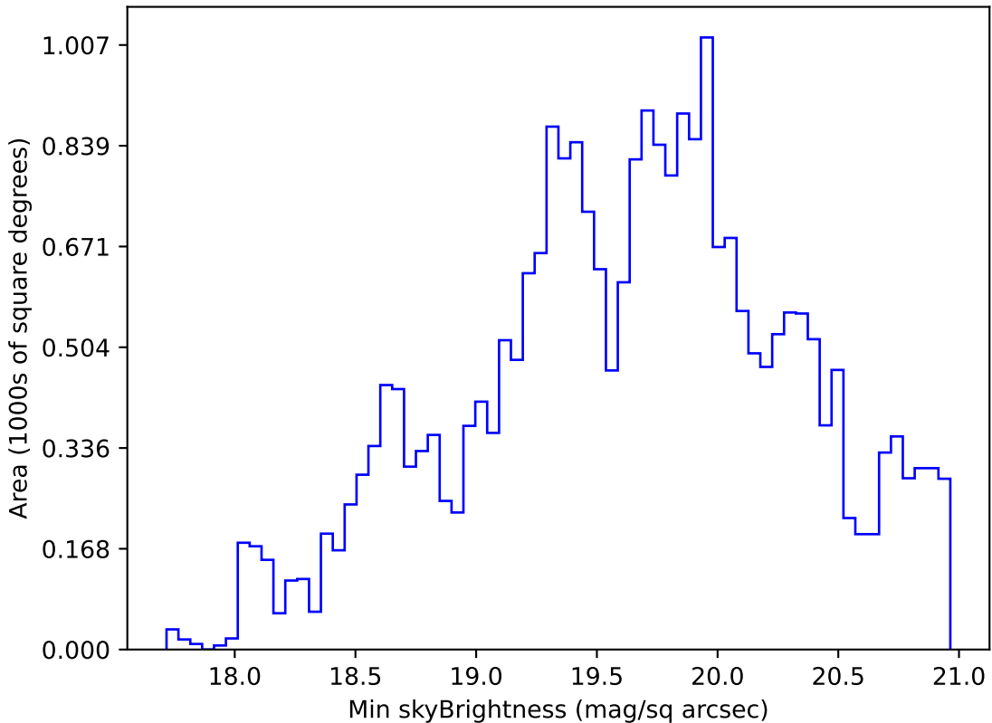
too_elab_r64_d3_giz_v3.4_10yrs Yr 1 r band: Min skyBrightness
