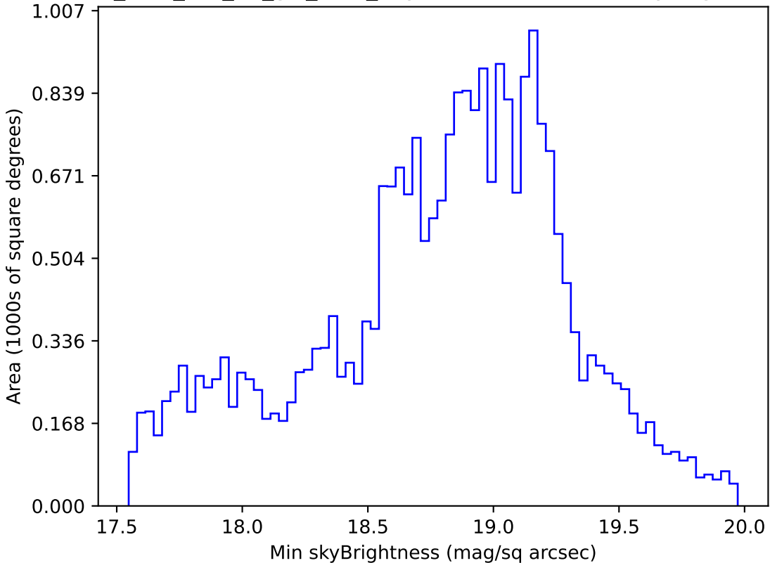
too_elab_r64_d3_giz_v3.4_10yrs Yr 1 i band: Min skyBrightness
