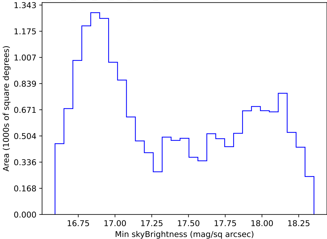
too_elab_r64_d3_giz_v3.4_10yrs WFD z band: Min skyBrightness
