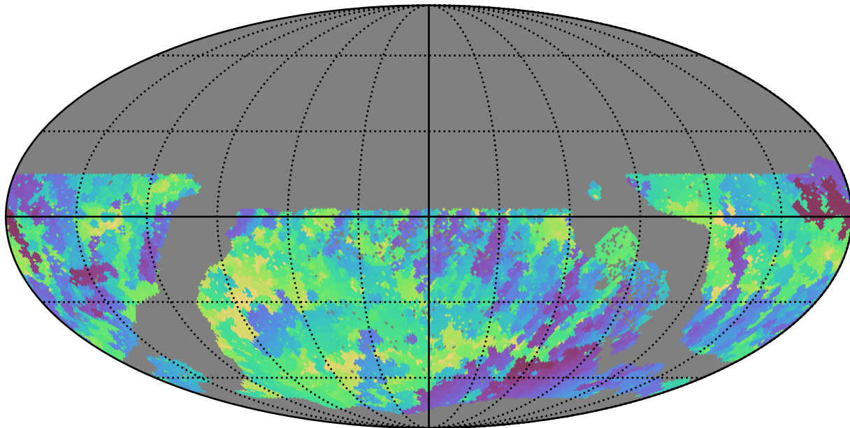
too_elab_r64_d3_giz_v3.4_10yrs WFD r band: Min skyBrightness
