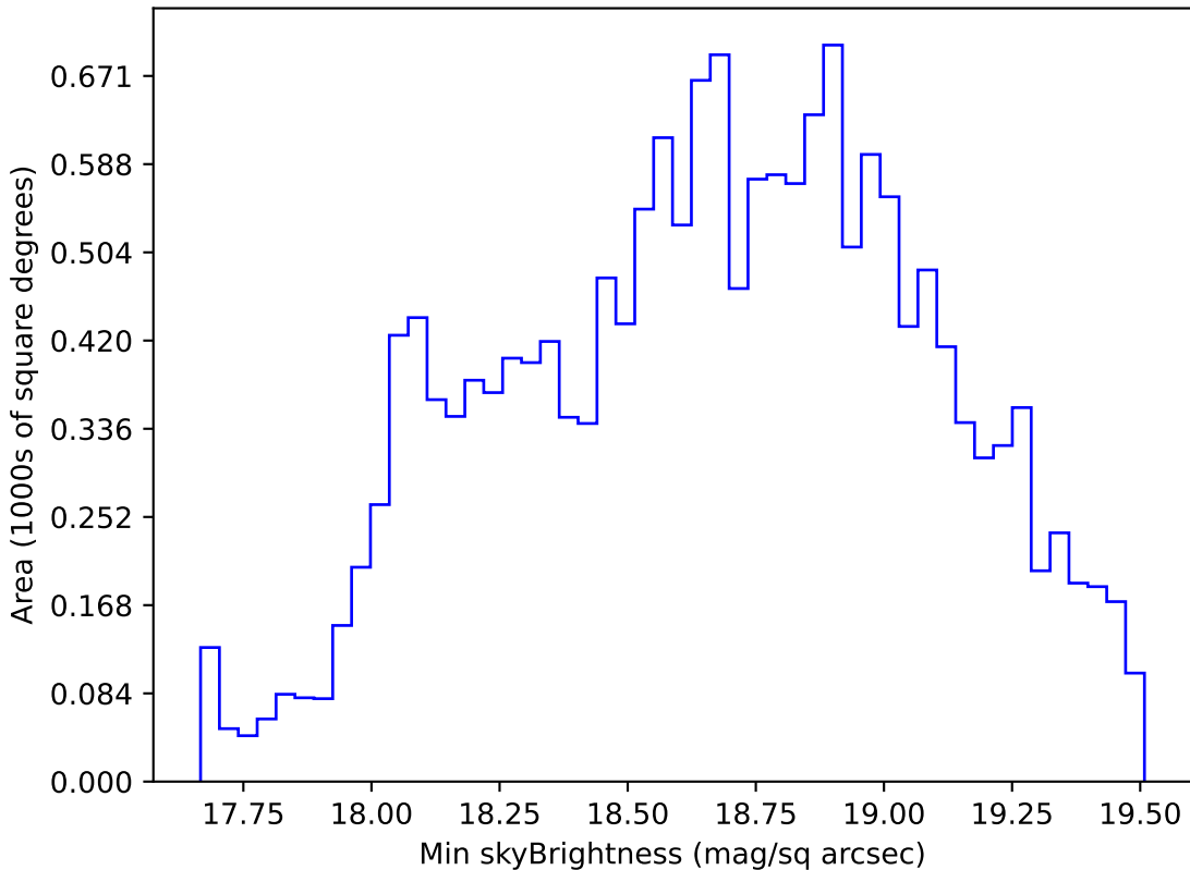
too_elab_r64_d3_giz_v3.4_10yrs WFD r band: Min skyBrightness
