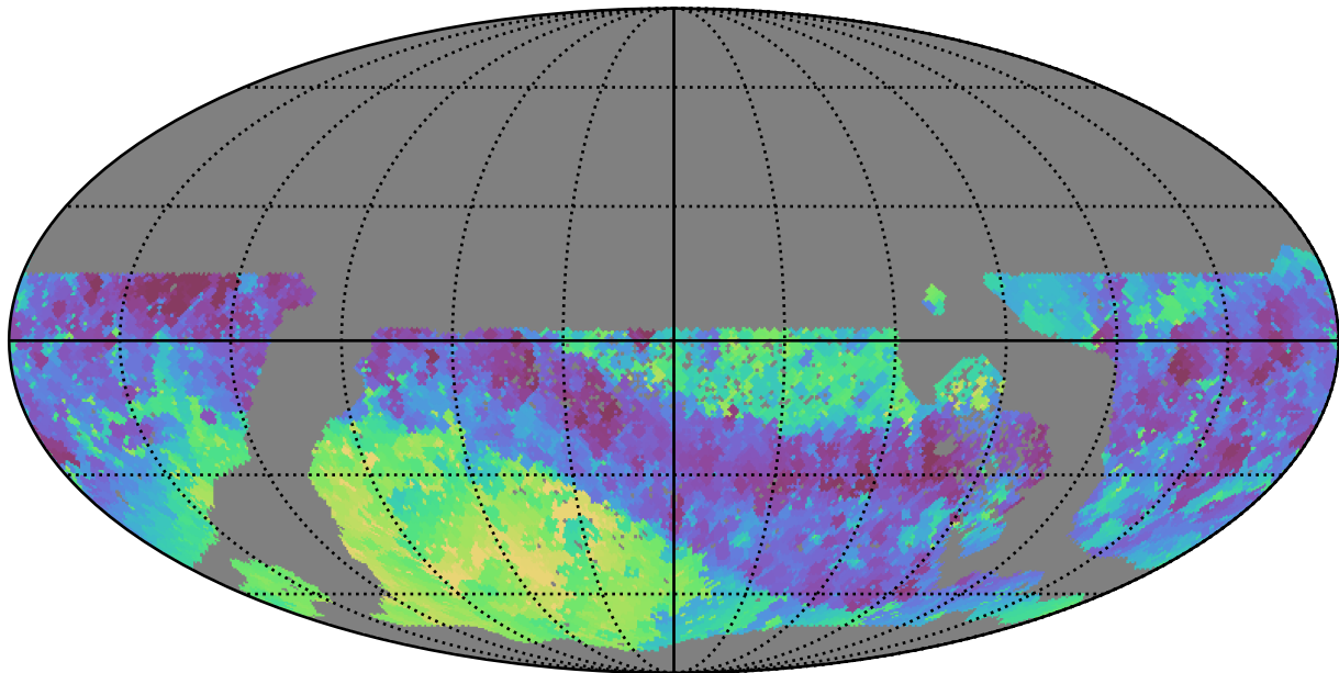
too_elab_r64_d3_giz_v3.4_10yrs WFD i band: Min skyBrightness
