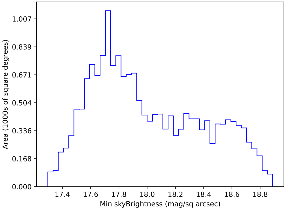
too_elab_r64_d3_giz_v3.4_10yrs WFD i band: Min skyBrightness
