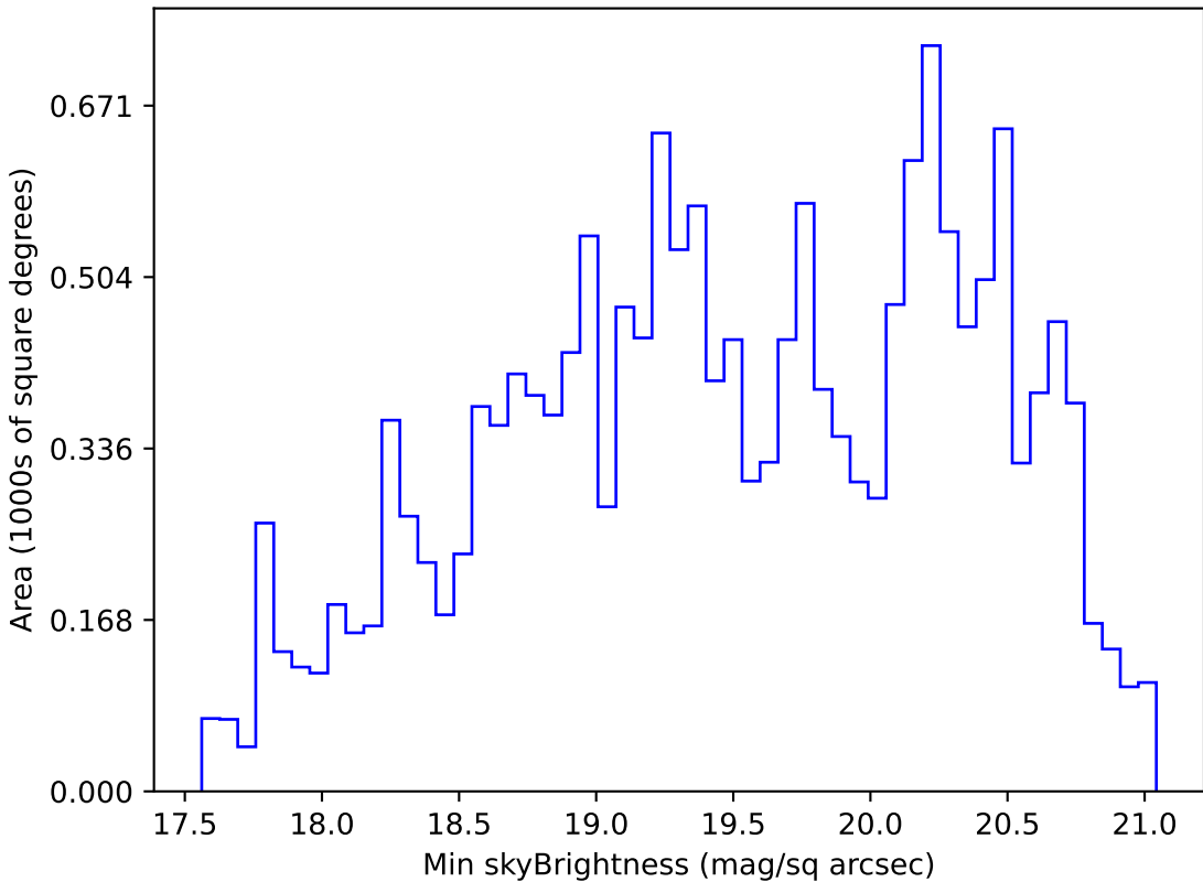
too_elab_r64_d3_giz_v3.4_10yrs WFD g band: Min skyBrightness
