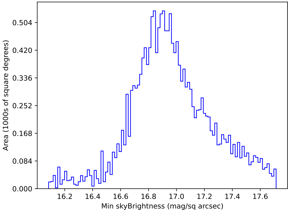
too_elab_r64_d3_giz_v3.4_10yrs WFD all bands: Min skyBrightness
