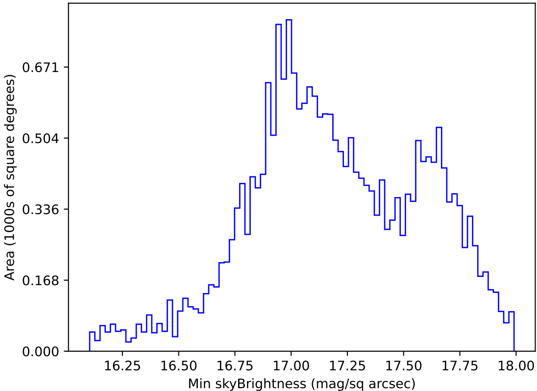
too_elab_r64_d3_giz_v3.4_10yrs All sky y band: Min skyBrightness
