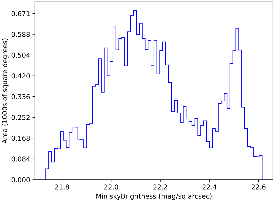
too_elab_r64_d3_giz_v3.4_10yrs All sky u band: Min skyBrightness
