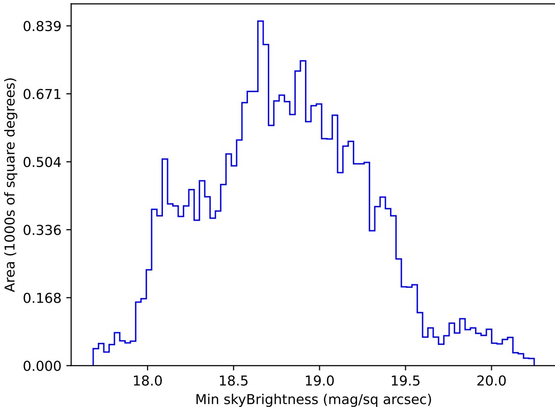
too_elab_r64_d3_giz_v3.4_10yrs All sky r band: Min skyBrightness
