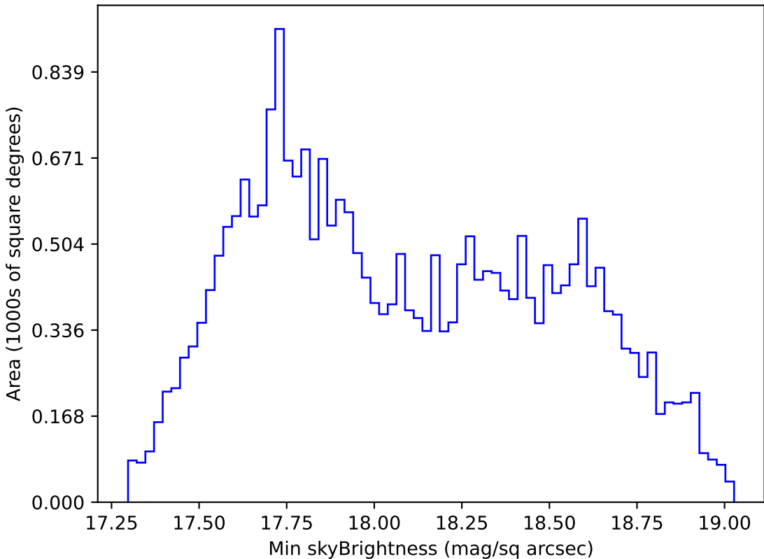
too_elab_r64_d3_giz_v3.4_10yrs All sky i band: Min skyBrightness
