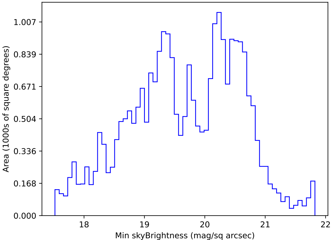
too_elab_r64_d3_giz_v3.4_10yrs All sky g band: Min skyBrightness
