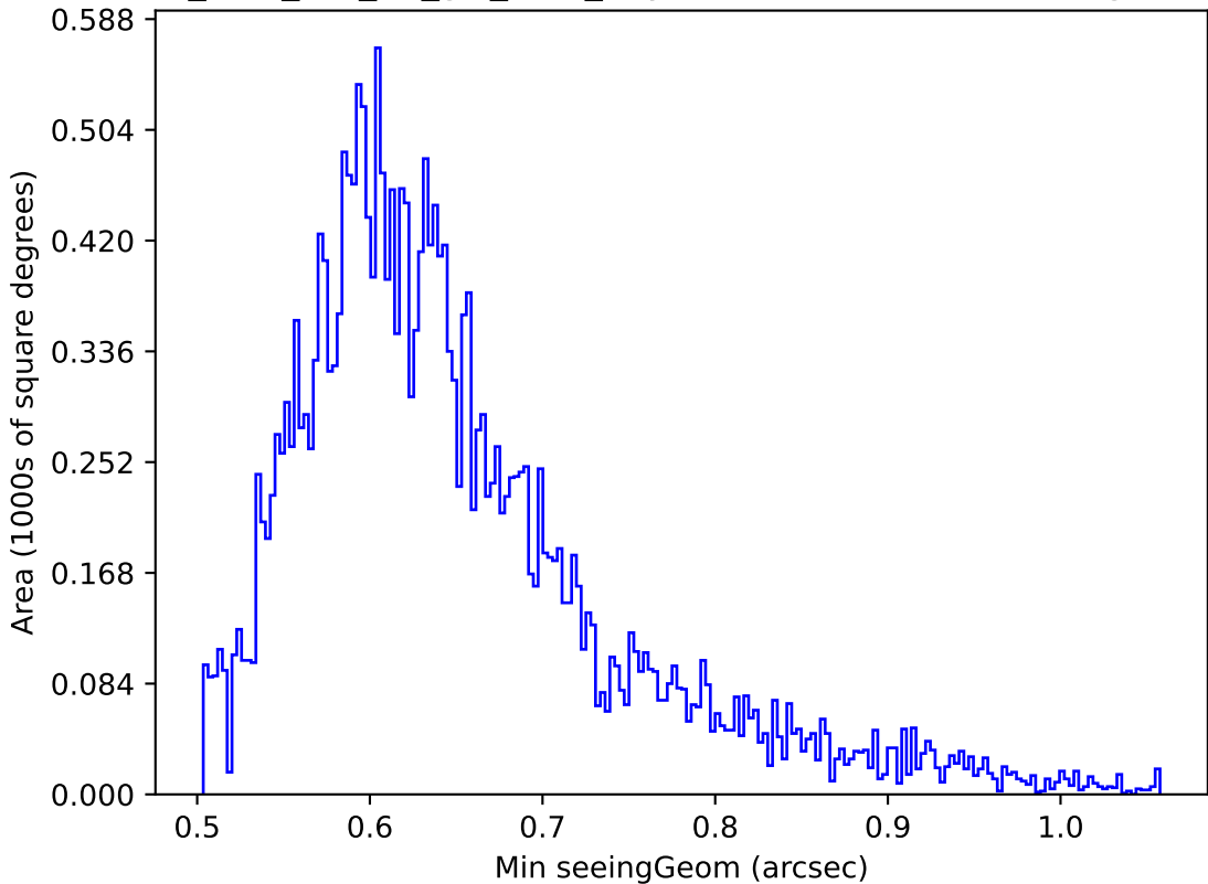
too_elab_r64_d3_giz_v3.4_10yrs Yr 1 z band: Min seeingGeom
