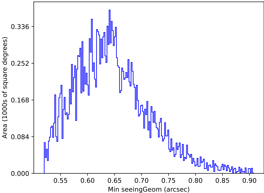
too_elab_r64_d3_giz_v3.4_10yrs Yr 1 y band: Min seeingGeom
