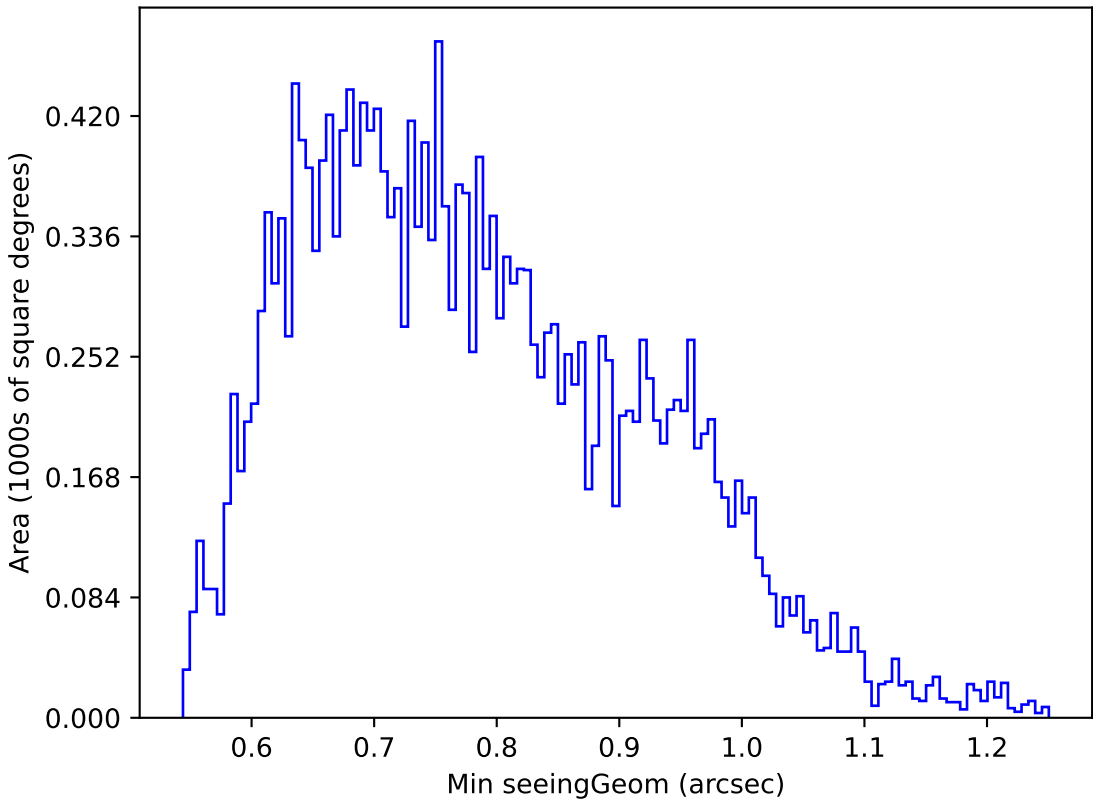
too_elab_r64_d3_giz_v3.4_10yrs Yr 1 u band: Min seeingGeom
