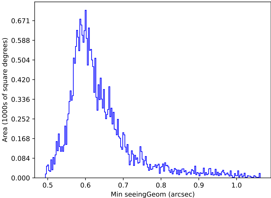
too_elab_r64_d3_giz_v3.4_10yrs Yr 1 i band: Min seeingGeom
