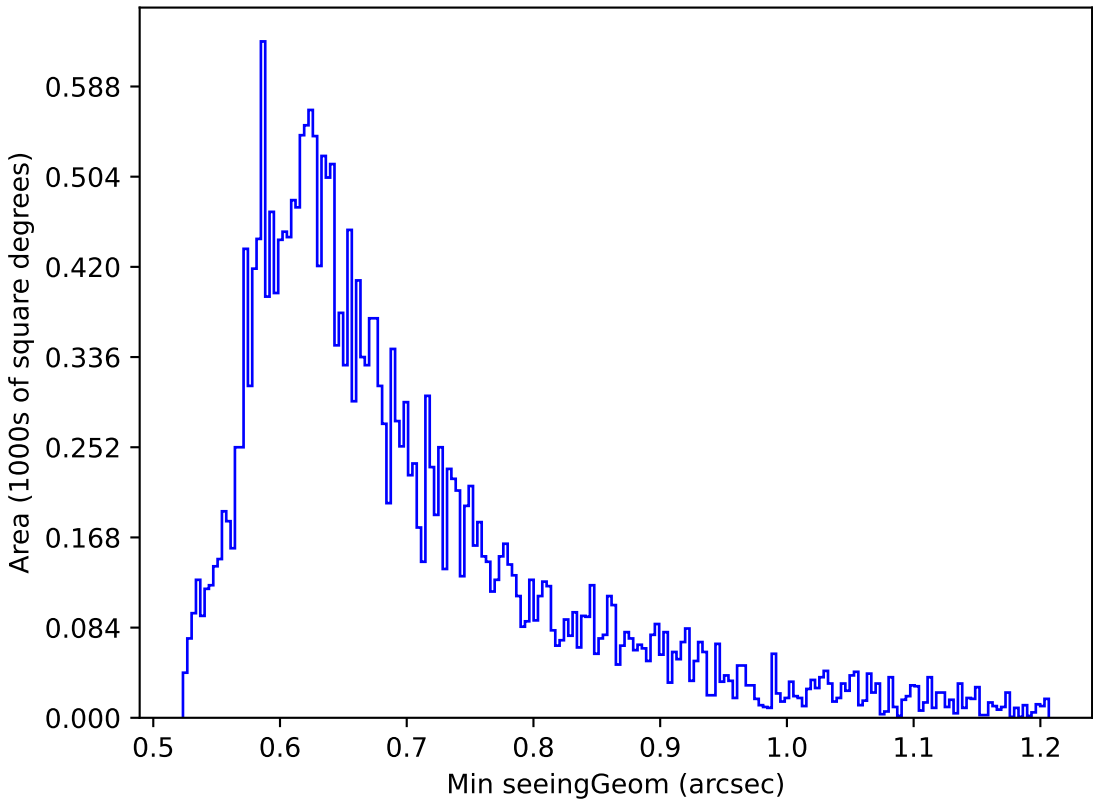
too_elab_r64_d3_giz_v3.4_10yrs Yr 1 g band: Min seeingGeom
