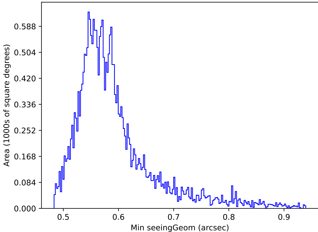
too_elab_r64_d3_giz_v3.4_10yrs Yr 1 all bands: Min seeingGeom
