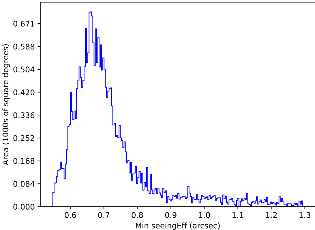
too_elab_r64_d3_giz_v3.4_10yrs Yr 1 r band: Min seeingEff
