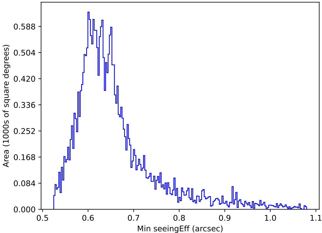
too_elab_r64_d3_giz_v3.4_10yrs Yr 1 all bands: Min seeingEff
