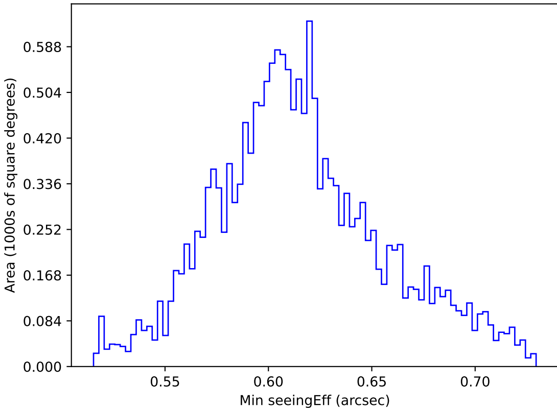
too_elab_r64_d3_giz_v3.4_10yrs WFD z band: Min seeingEff
