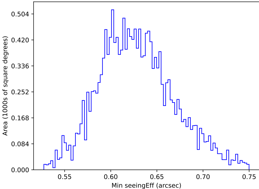
too_elab_r64_d3_giz_v3.4_10yrs WFD y band: Min seeingEff
