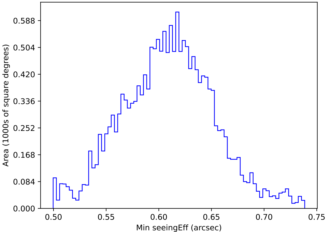
too_elab_r64_d3_giz_v3.4_10yrs WFD r band: Min seeingEff
