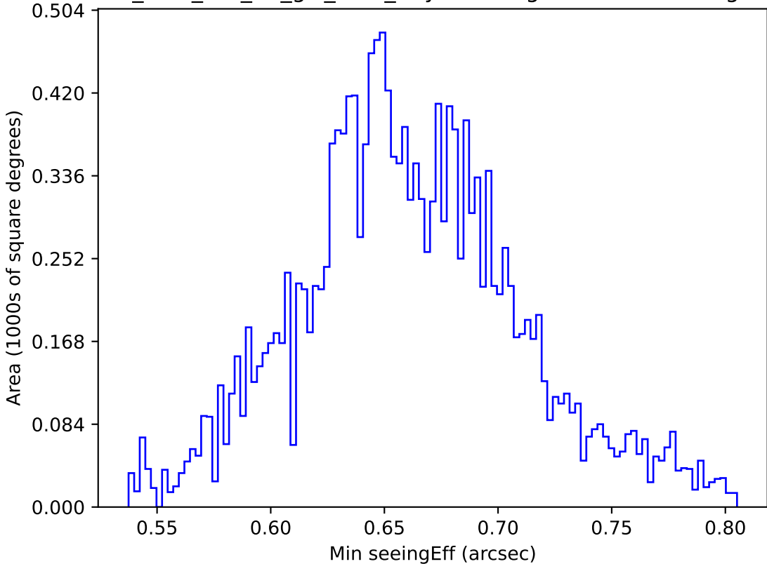
too_elab_r64_d3_giz_v3.4_10yrs WFD g band: Min seeingEff
