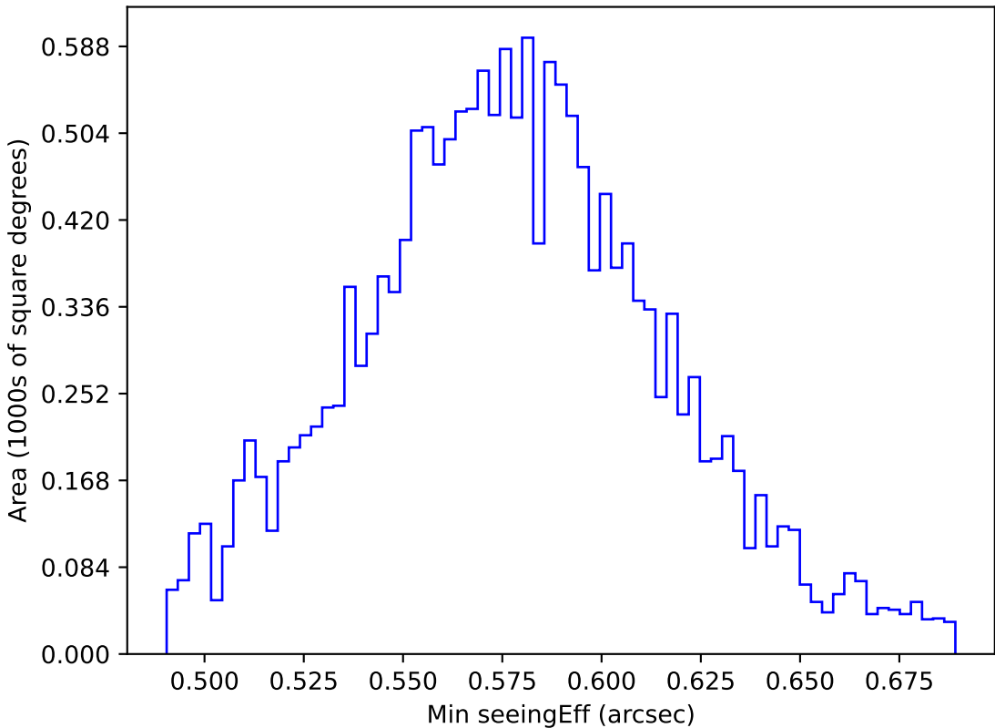
too_elab_r64_d3_giz_v3.4_10yrs WFD all bands: Min seeingEff
